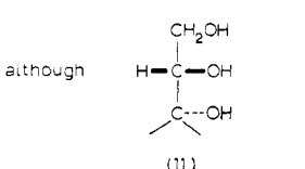
17,20 \alpha ,21-triol (20 S )
