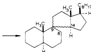
14(8 \rightarrow 9 \xi ) abeo -5 \alpha -Cholestane†
