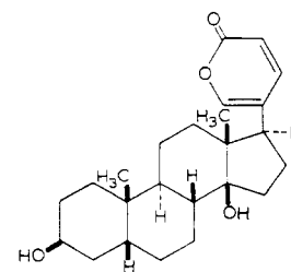
3 \beta ,14-Dihydroxy-5 \beta ,14 \beta -bufa-20,22-dienolide (= bufalin*)
