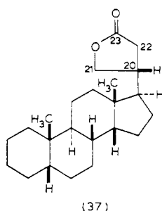
5 \beta ,14 \beta -Cardanolide
