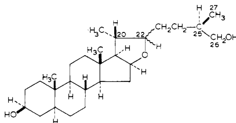
(58) (20 S ,22ξ,25 R )-5α-Furostan-3β,26-diol (Dihdropseudotigogenin*)
