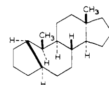
5(10 \rightarrow 1 \alpha H) abeo -5 \alpha -Androstane**
