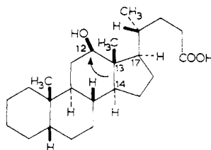
12 \beta -Hydroxy-5 \beta -cholan-24-oic acid
