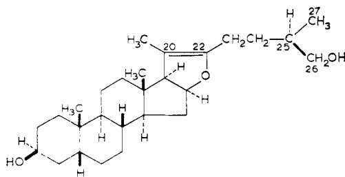
(59) (25 S )-5β-Furost-20(22)-en-3β,26-diol (Pseudosarsapogenin*)
