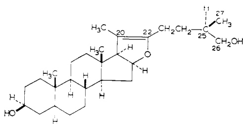
(57) (25 R )-5α-Furost-20(22)-en-3β,26-diol (Pseudotigogenin*)
