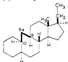
(86) B(9a) -Homo-19-nor-5 \alpha ,10 \alpha (H)-pregnane*
