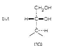
20 \alpha ,21-diol (20 R )
