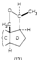
(20 S )-18,20-Epoxypregnane ( \equiv 20 \alpha )
