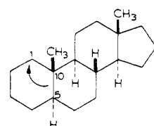
5 \alpha -Androstane
