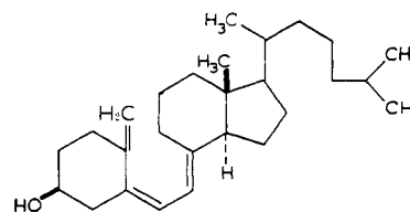
(94) 9,10- Seco -5,7,10(19)-cholestatrien-3 \beta -ol (trivial name: cholecalciferol**)
