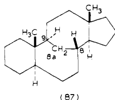
(87) BC(8a) -Homo-5 \alpha -androstane
