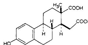
(93) 3-Hydroxy-16,17- seco -1,3,5(10)-estratriene-16,17-dioic acid
