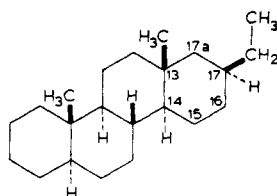
(89) 17 \beta -Ethyl- D -homo-5 \alpha -androstane
