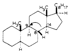
5 \alpha -Cholestane
