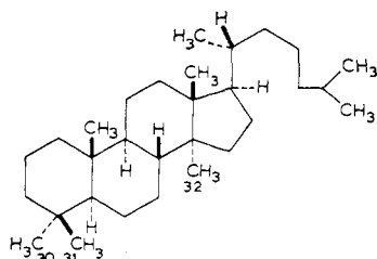
(27) 5α-Lanostane
